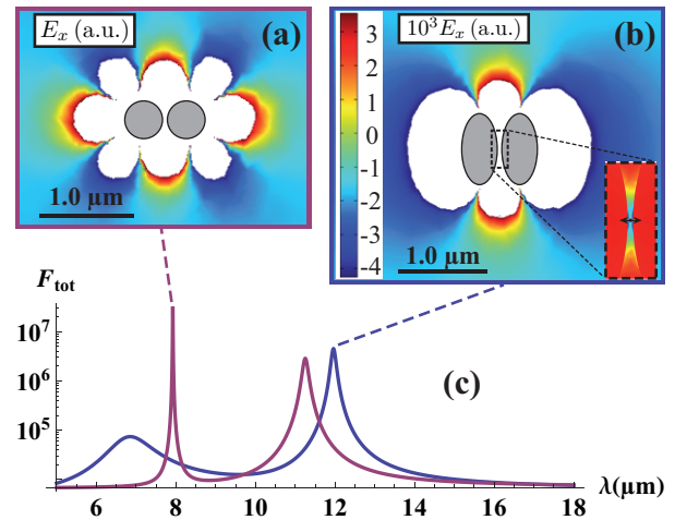
Figure 2: (color online) (a) & (c) Two circular graphene elements cause a strong enhancement of the total emission rate F_{\text{tot}} for a dark antenna mode at \lambda \approx 7.9 \mu\text{m} ( \nu \approx 38 \text{ THz} ). To visualize the field outside the antenna, the colormap has been truncated (white regions). (b) & (c) The antenna with two elliptical elements exhibits by far the strongest F_{\text{tot}} for the desired dipolar mode at \lambda \approx 12 \mu\text{m} ( \nu \approx 26.6 \text{ THz} ). The scale shown in (b) applies for all field plots with order-of-magnitude rescalings.
